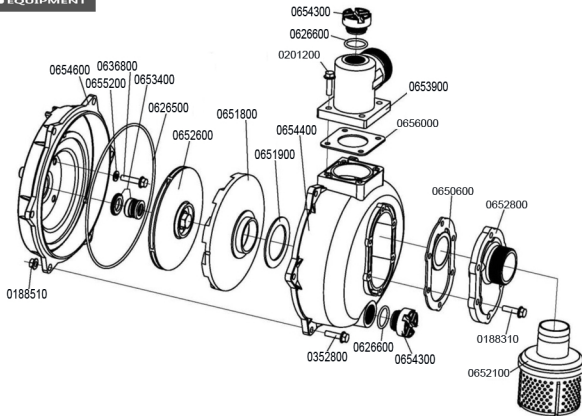
LE71196-50H(HP20A) PUMP BODY PART
