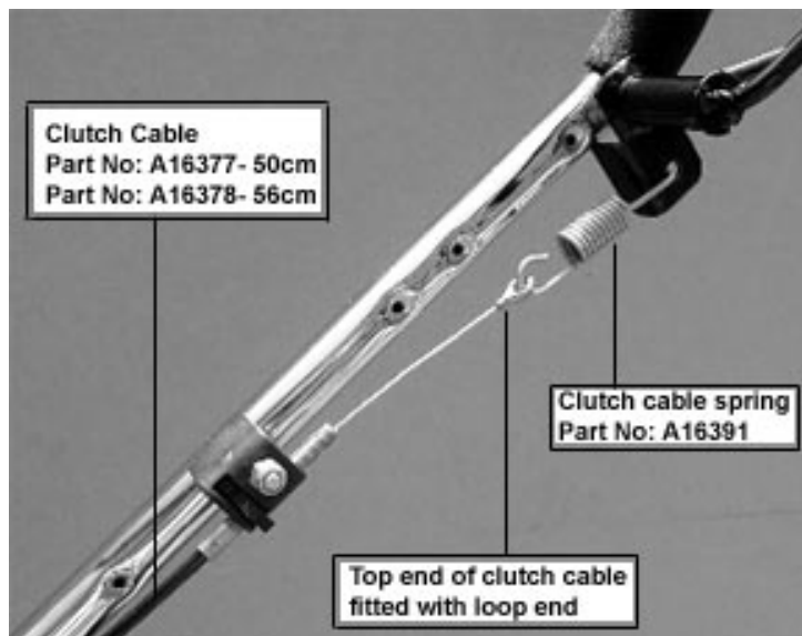
Clutch cable mounting on upper handle bars
