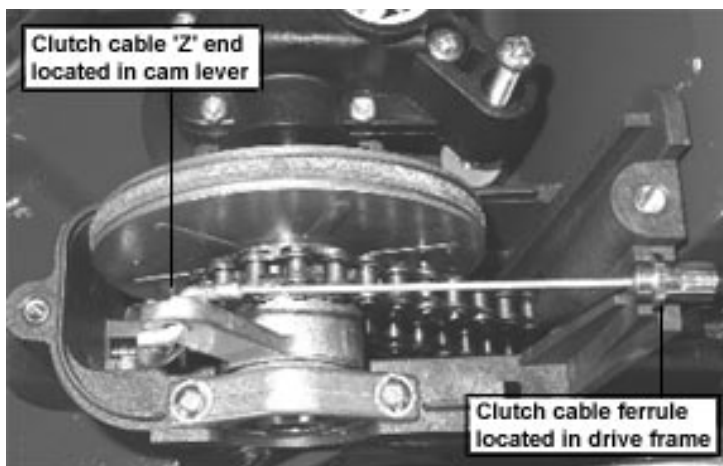
Clutch cable attachment to cam lever
